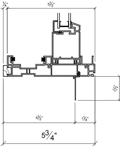
4 5/8" JAMB
