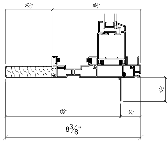
7 1/8" JAMB
