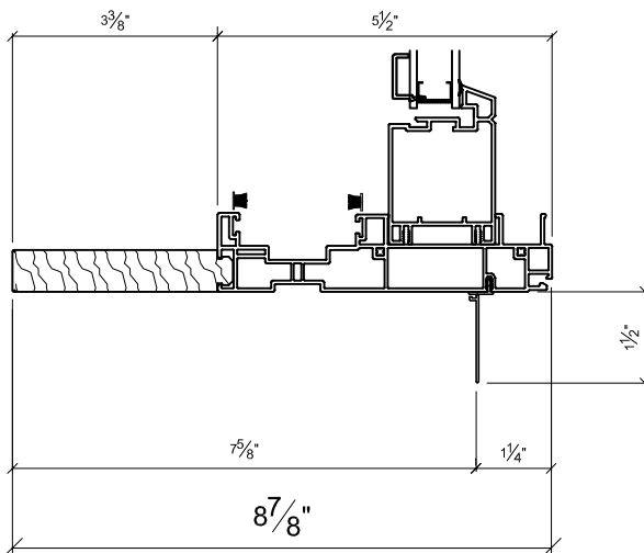
7 5/8" JAMB
